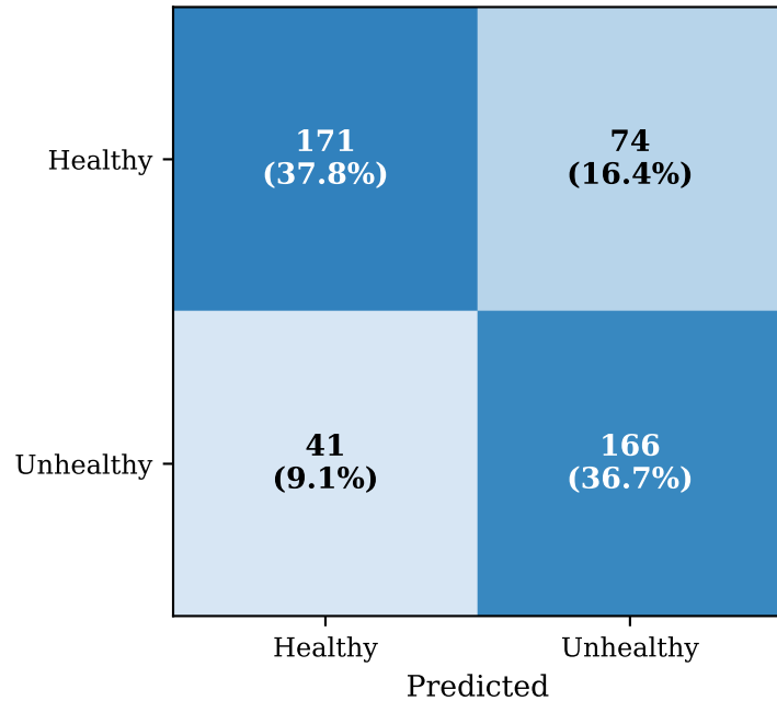
CDS-only (74.6%)
