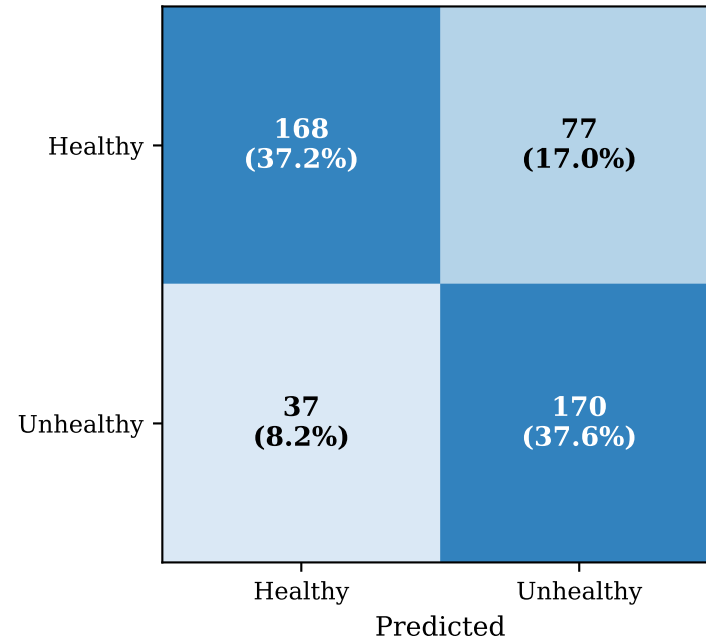
Cascade(ANN) (74.8%)
