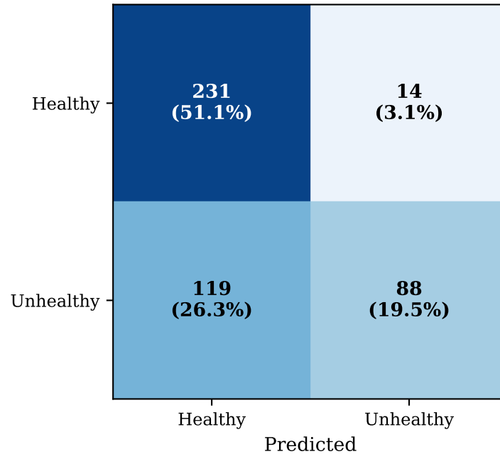
ANN-only (70.6%)
