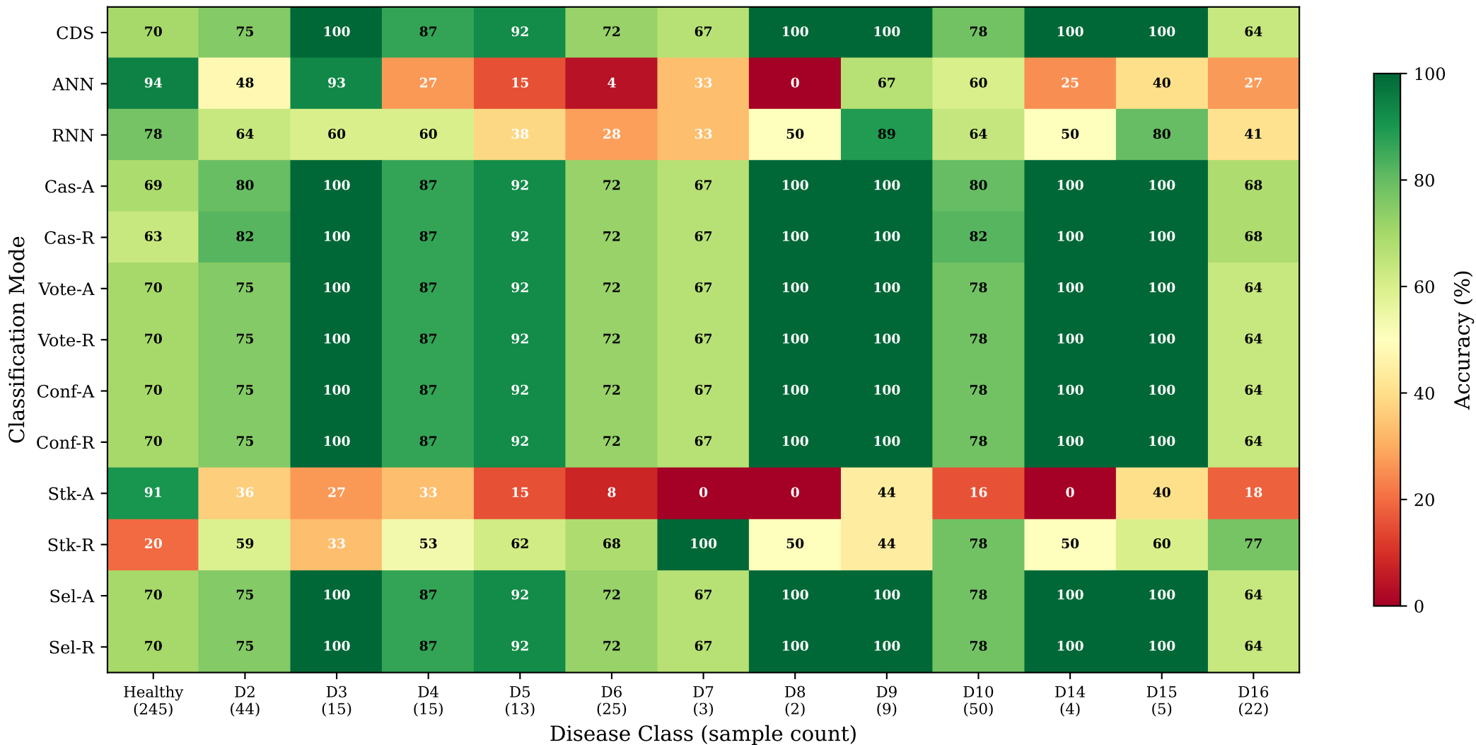
Fig. 7: Per-Class Accuracy Heatmap (% correct per disease class)
