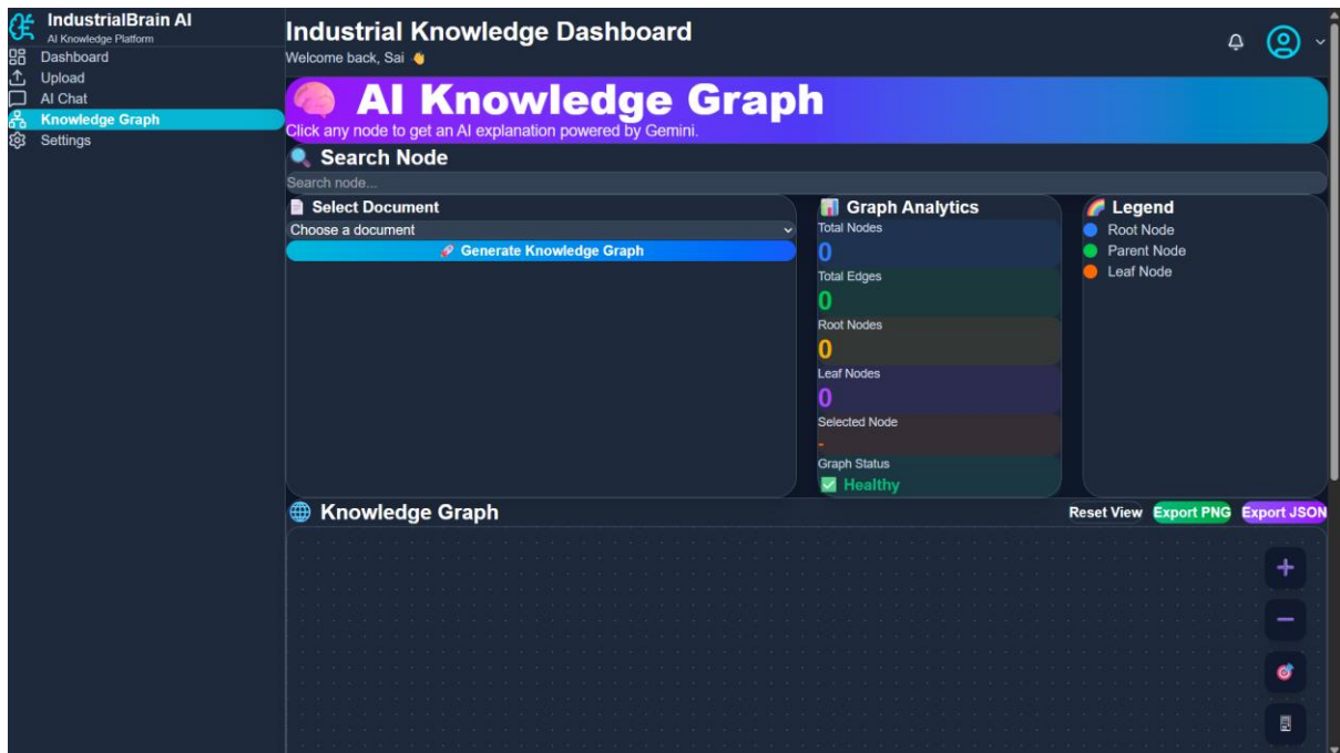
Figure 12.18: Knowledge Overview
