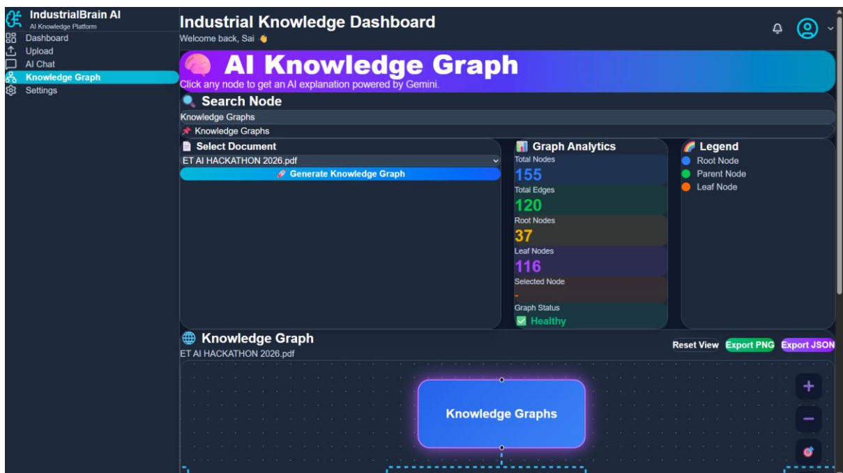
12.19: Node Search
