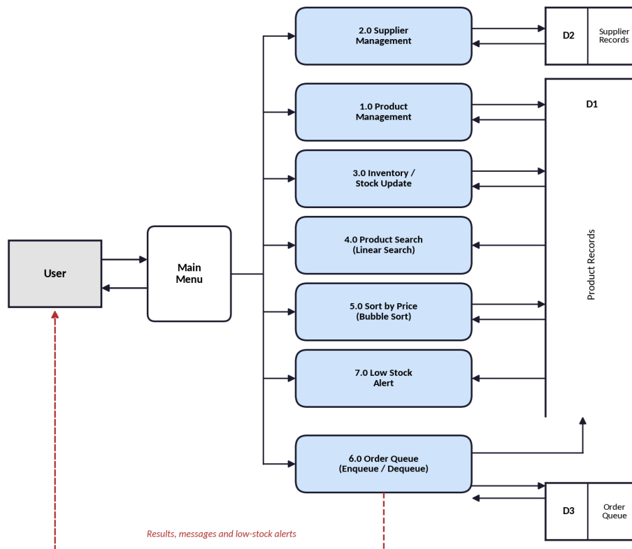
Fig 3.2 Level 1 Data Flow Diagram showing the seven modules and the three data stores
