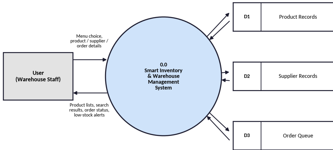
Fig 3.1 Level 0 Data Flow Diagram of the Smart Inventory and Warehouse Management System
