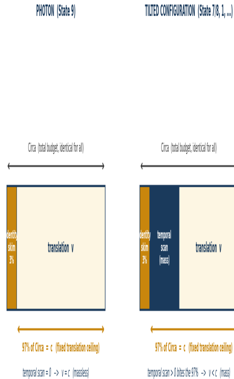
Figure 1 - The Budget of Circa. The three-percent identity skim comes off the top of the one universal budget; the remaining ninety-seven percent is the fixed translation ceiling c . The photon (left) runs zero temporal scan and commits the whole ninety-seven percent to translation; a tilted configuration (right) runs a temporal scan that bites into the ninety-seven percent, and that bite is mass.
