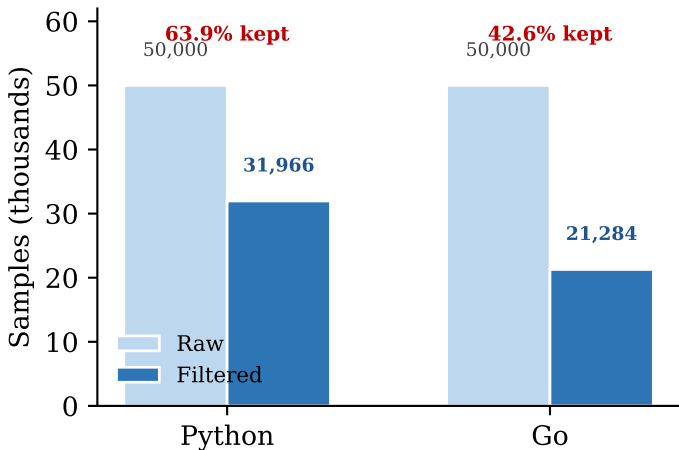
Pipeline input cap vs. retained samples
