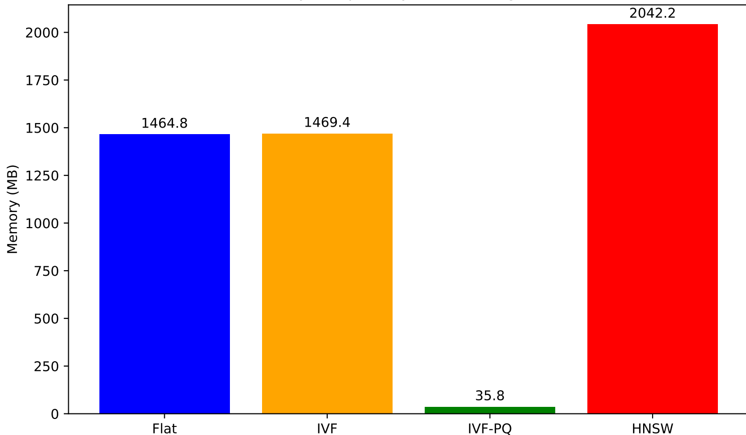
Memory Footprint by Index Configuration
