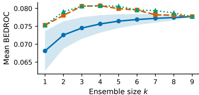
a Early recognition
