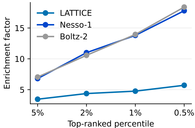
Mean enrichment
