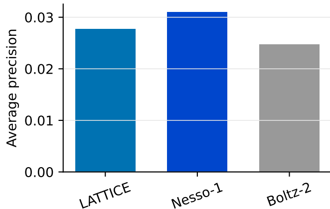
Mean AP
