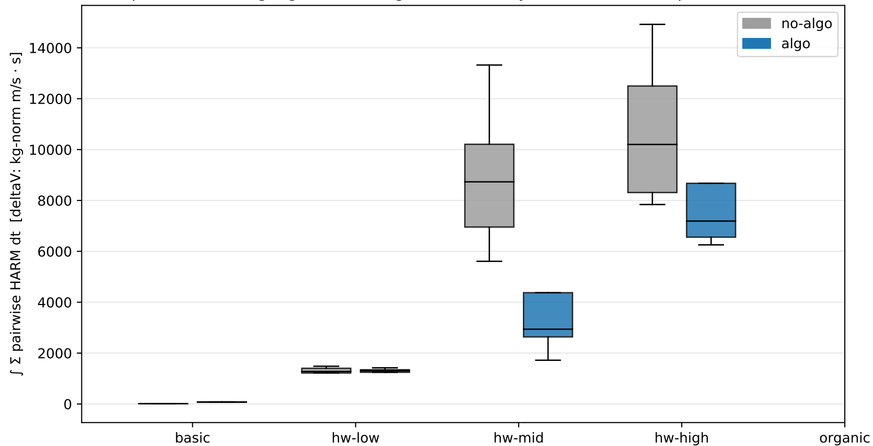
Cooperative-braking algorithm: integrated HARM by scenario (box = spread over seeds)
