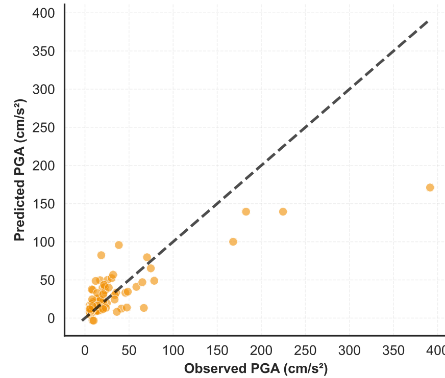
(f) LightGBM Maximum PGA R^2=0.645 , RMSE=30.71
