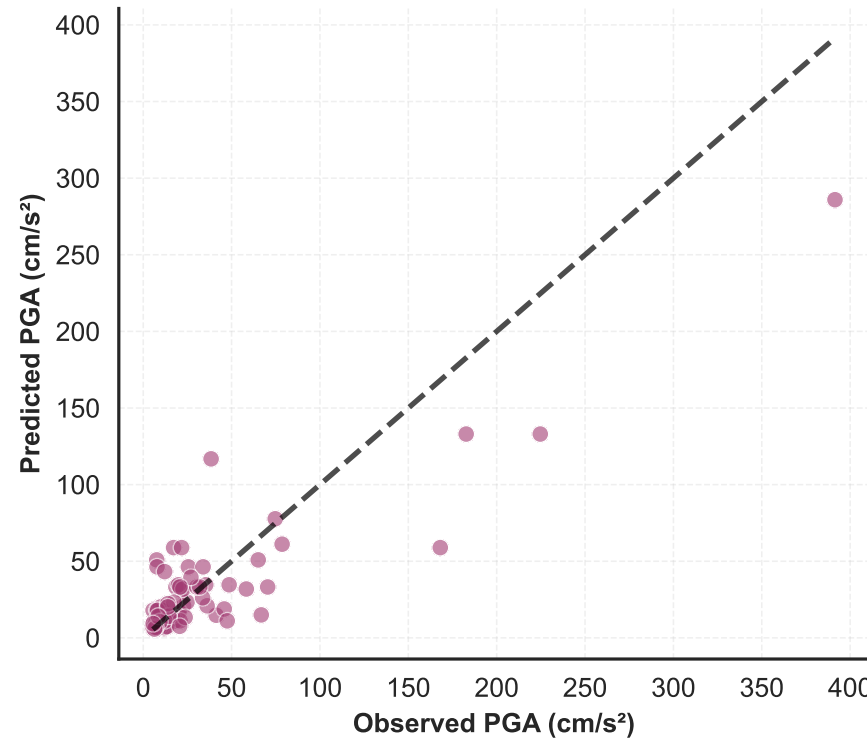
(e) Decision Tree Maximum PGA R^2=0.761 , RMSE=25.21
