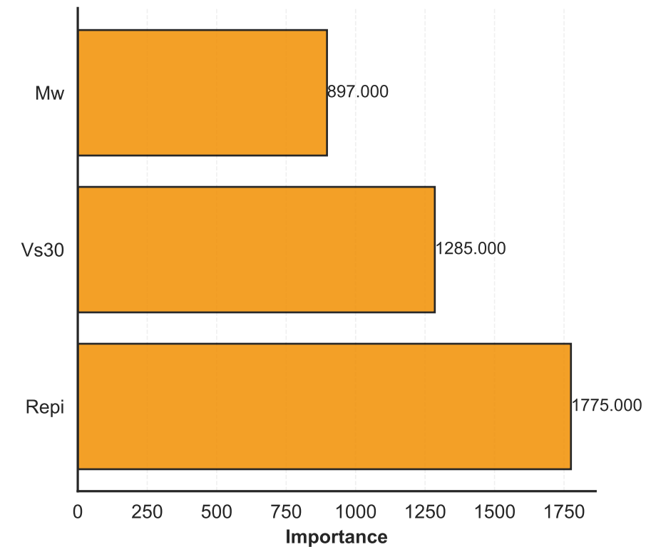
(f) LightGBM Maximum PGA
