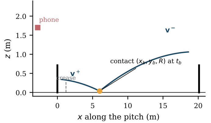
Fig. 1. The model. A delivery is two gravity parabolas joined at the contact point, whose height above the pitch is the ball radius. The phone sits behind one set of stumps, so the ball travels nearly along the optical axis and its depth is the least observable coordinate.
