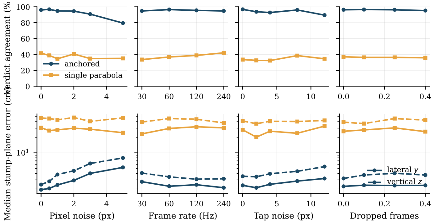
Fig. 2. Experiment 1. Top: verdict agreement against each measurement factor. Bottom: median stump-plane error, lateral (solid) and vertical (dashed), for the anchored estimator (blue) and the single parabola (orange). The anchored estimator is flat in every factor until pixel noise reaches several pixels.
