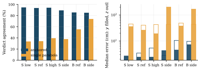
Fig. 3. Experiment 1, camera placement. S is the striker's end, B the bowler's. Left: agreement, both estimators. Right: median lateral (filled) and vertical (outline) stump-plane error, logarithmic axis.
