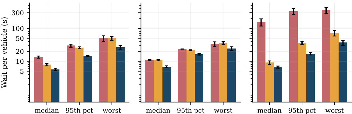
Asymmetric demand (1278 veh/h)
