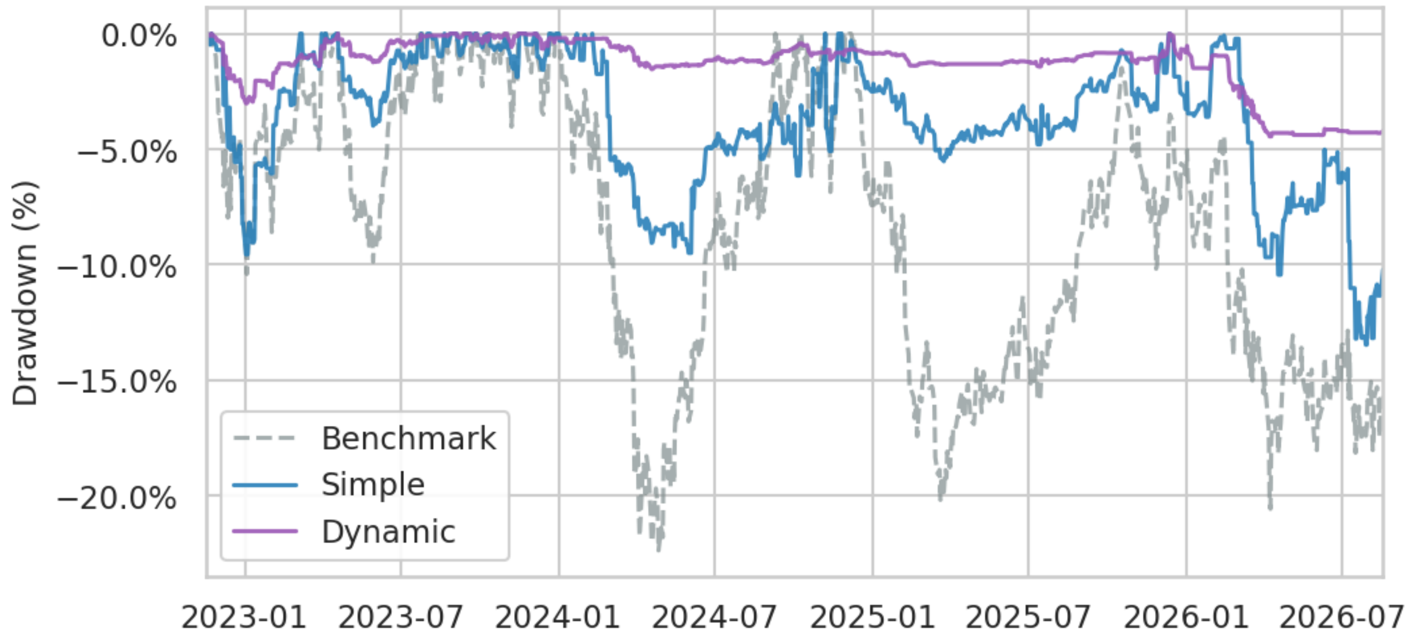
Portfolio Drawdown Comparison
