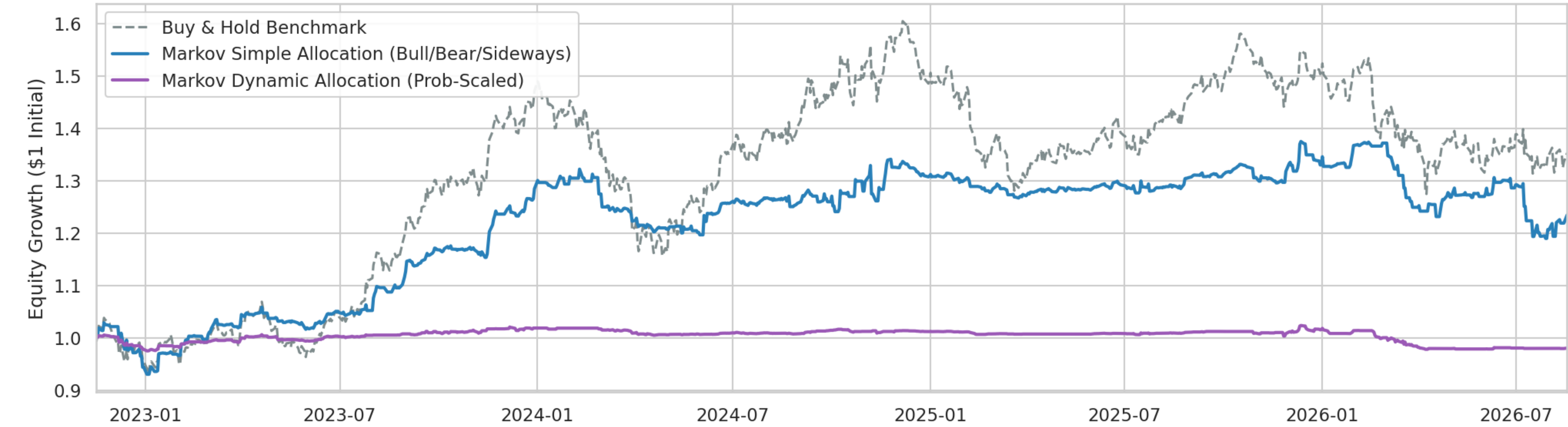
Portfolio Growth Comparison (Out-of-Sample Walk-Forward Period)
