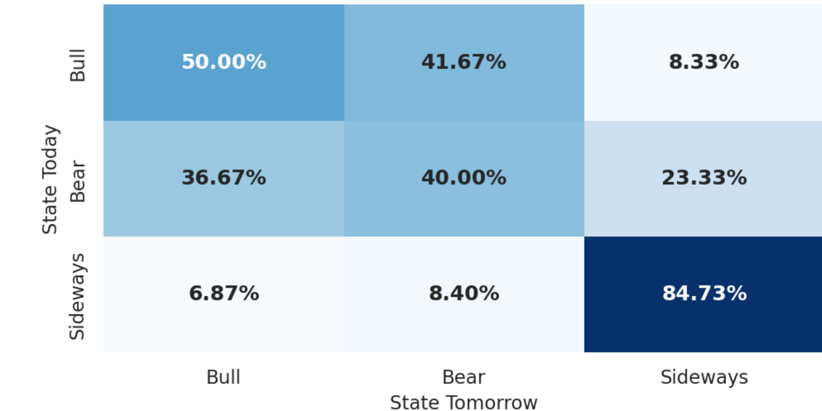
Decoded Transition Matrix (P)
