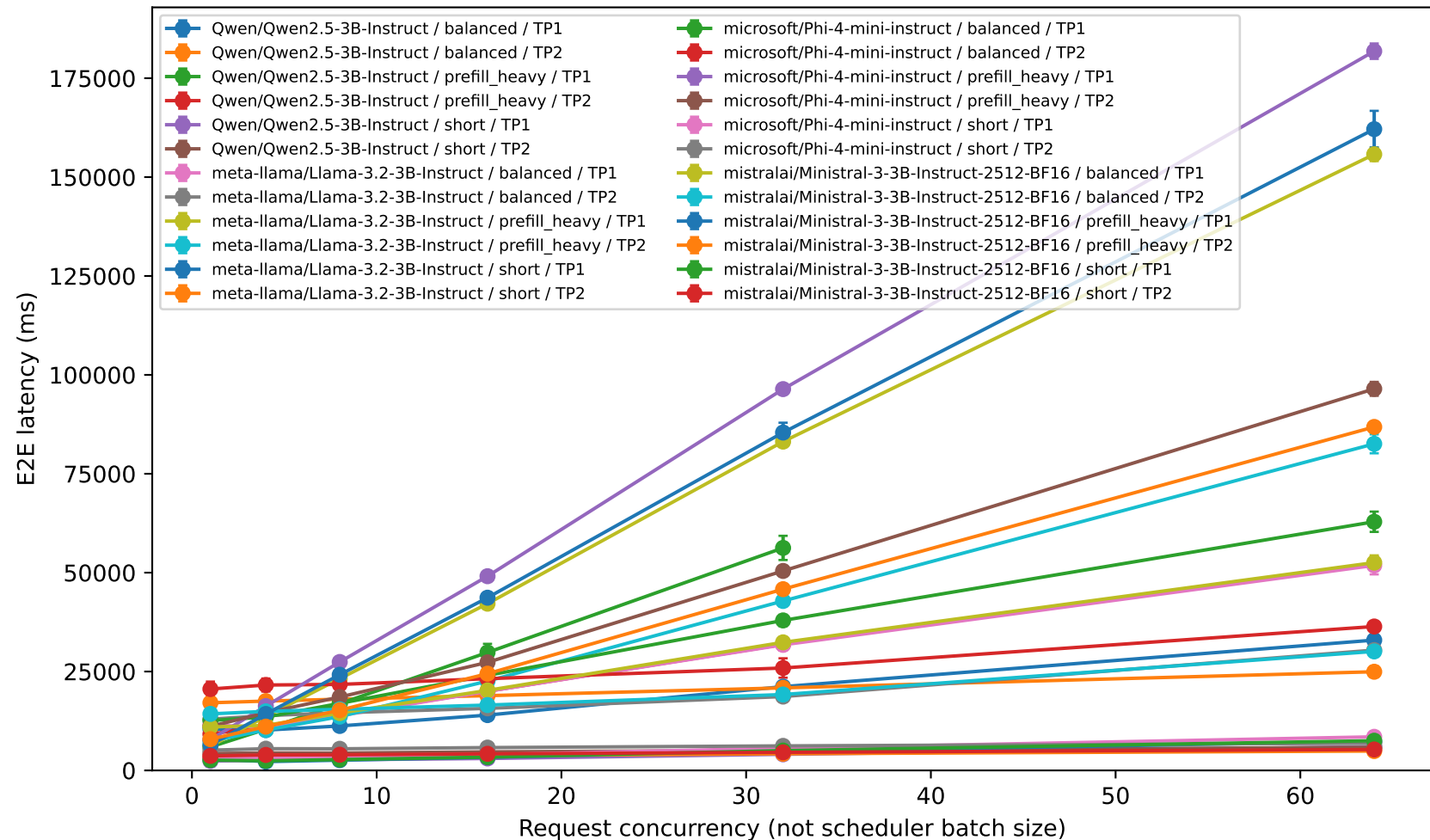
M4 measured serving results (n \geq 5 independent repetitions; 95% CI)
