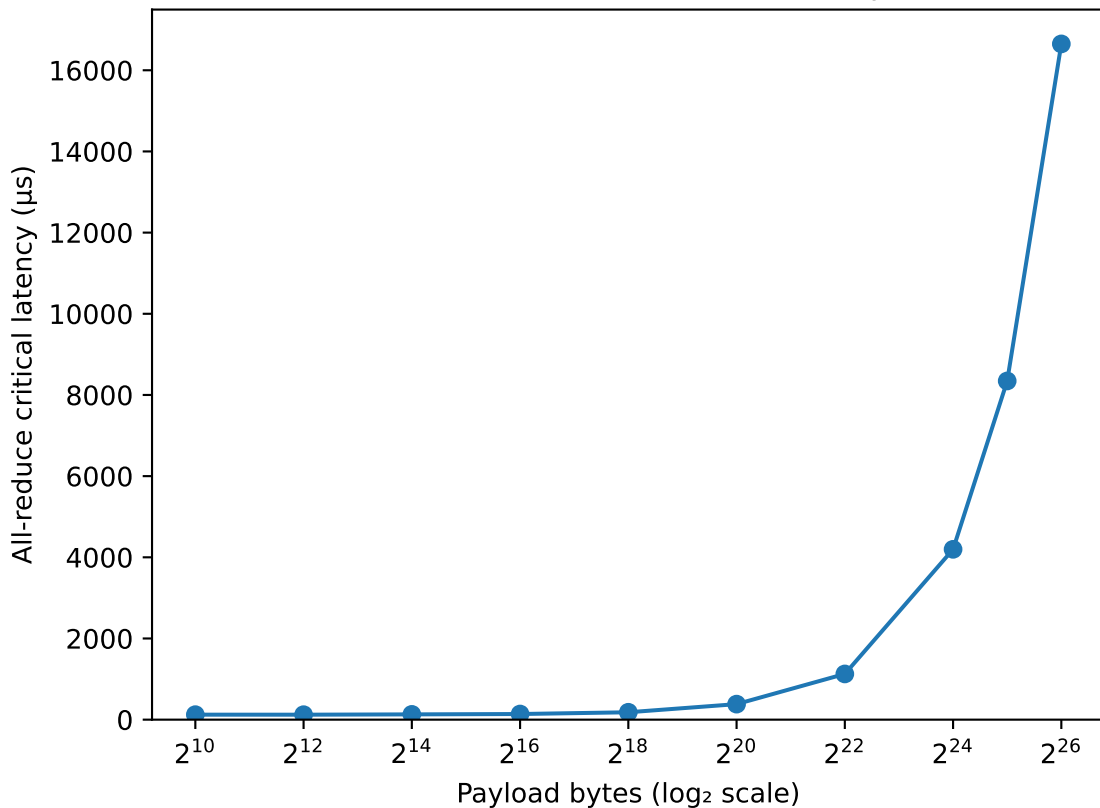
M3 measured two-rank NCCL all-reduce (n=5 repetitions; 95% CI)
