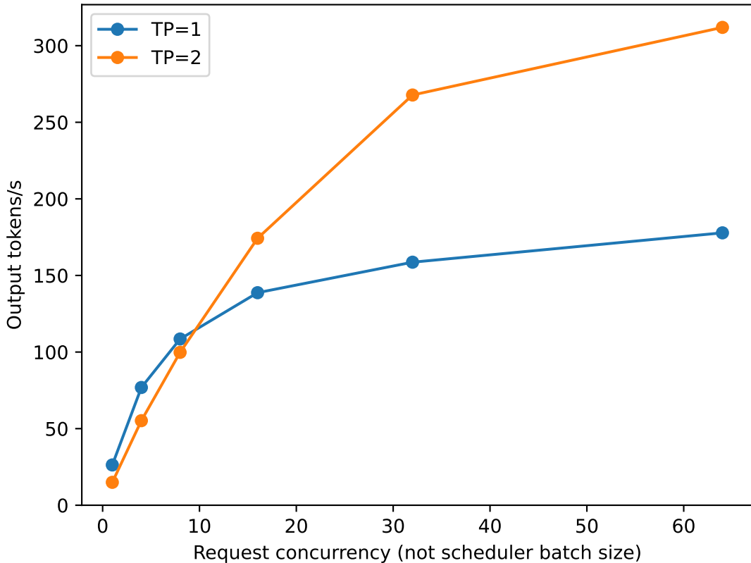
M2 measured Qwen concurrency crossover (n=1 run/cell)
