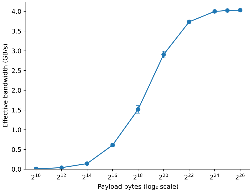
M3 measured two-rank NCCL all-reduce (n=5 repetitions; 95% CI)
