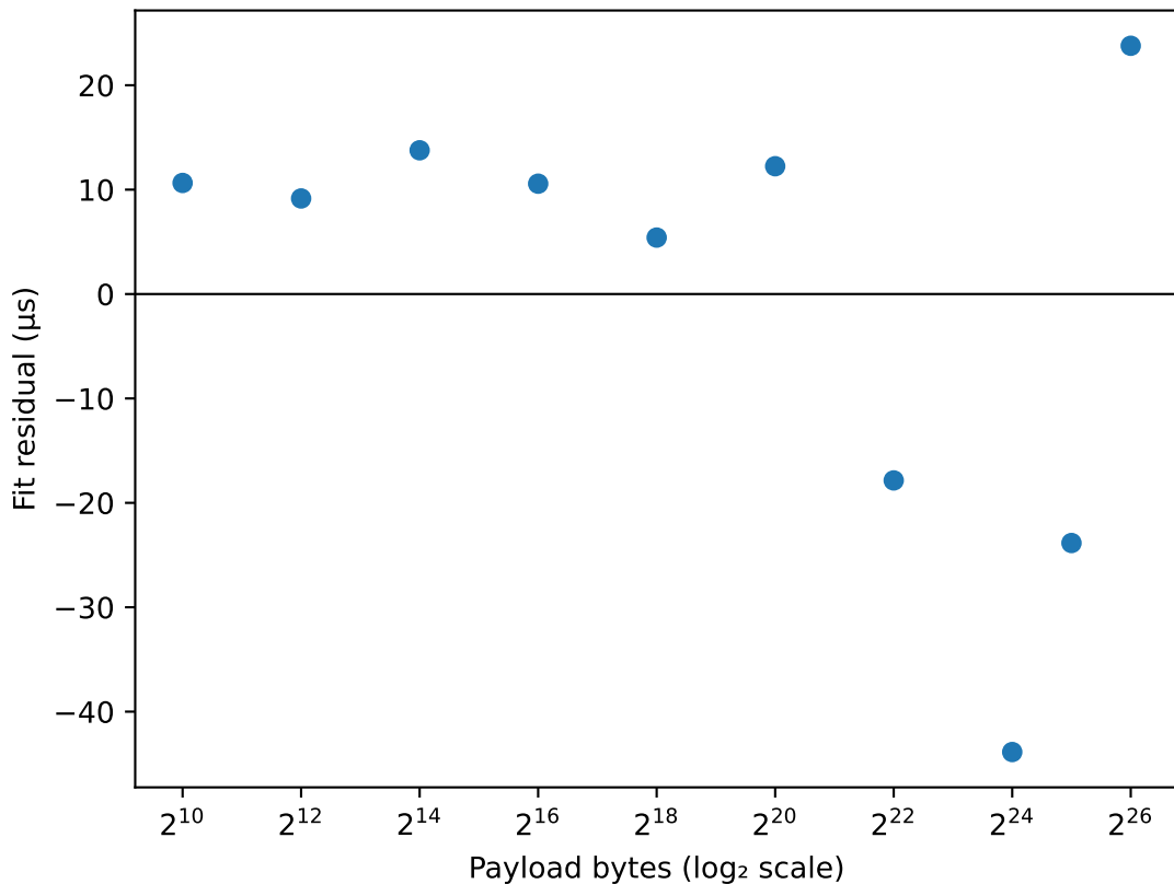
M3 all-reduce fit residuals
