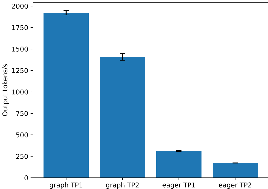
M1 measured low-load TP behavior (n=5 trials/cell; \pm 1 SD)
