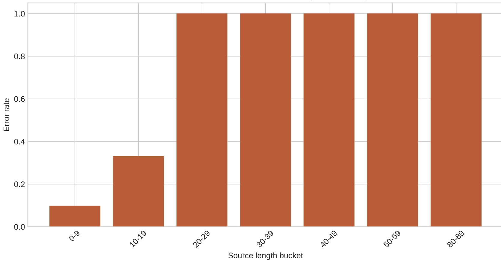
Arabic-with-harakat to Arabizi error by source length
