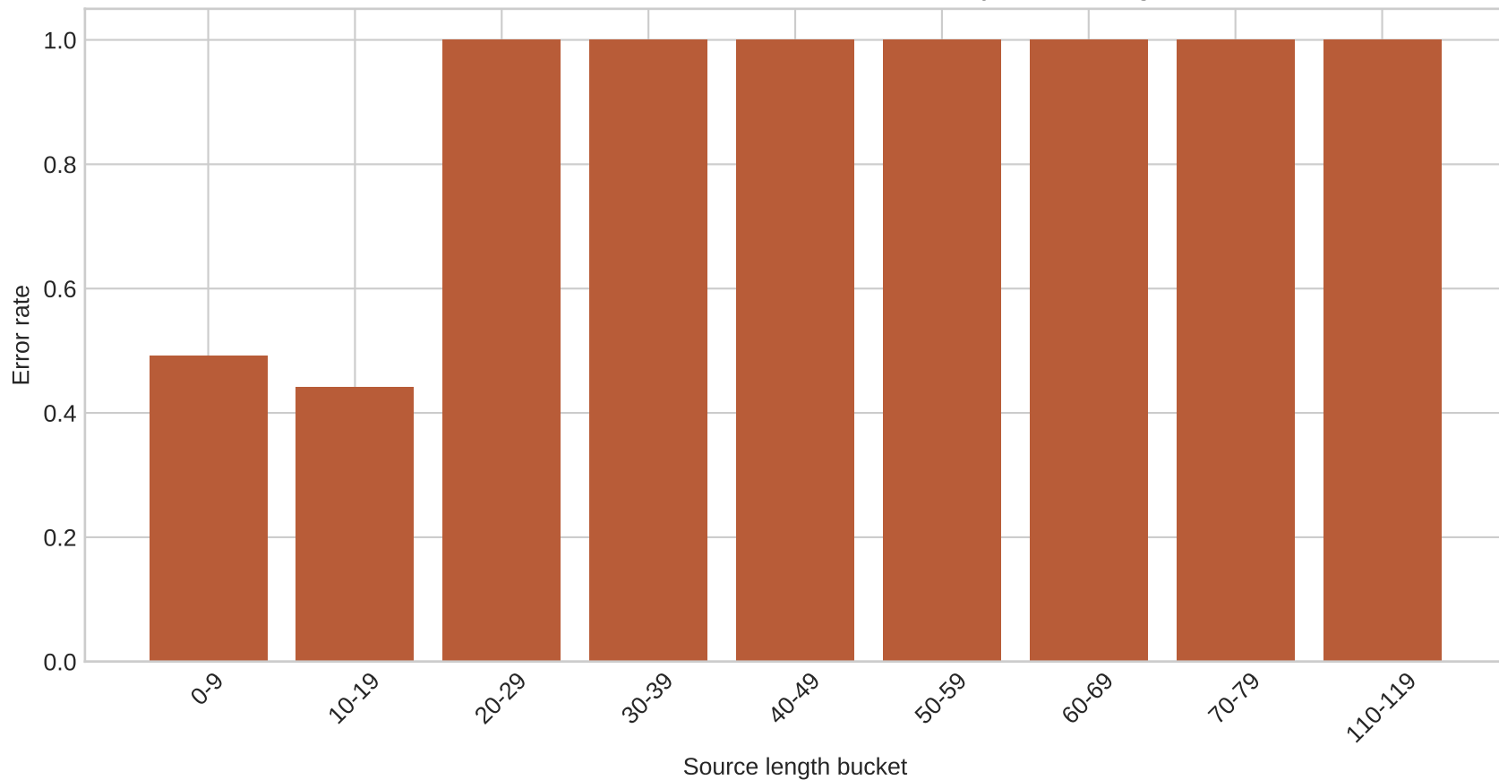
Arabic-with-Levanti-harakat to Arabizi error by source length
