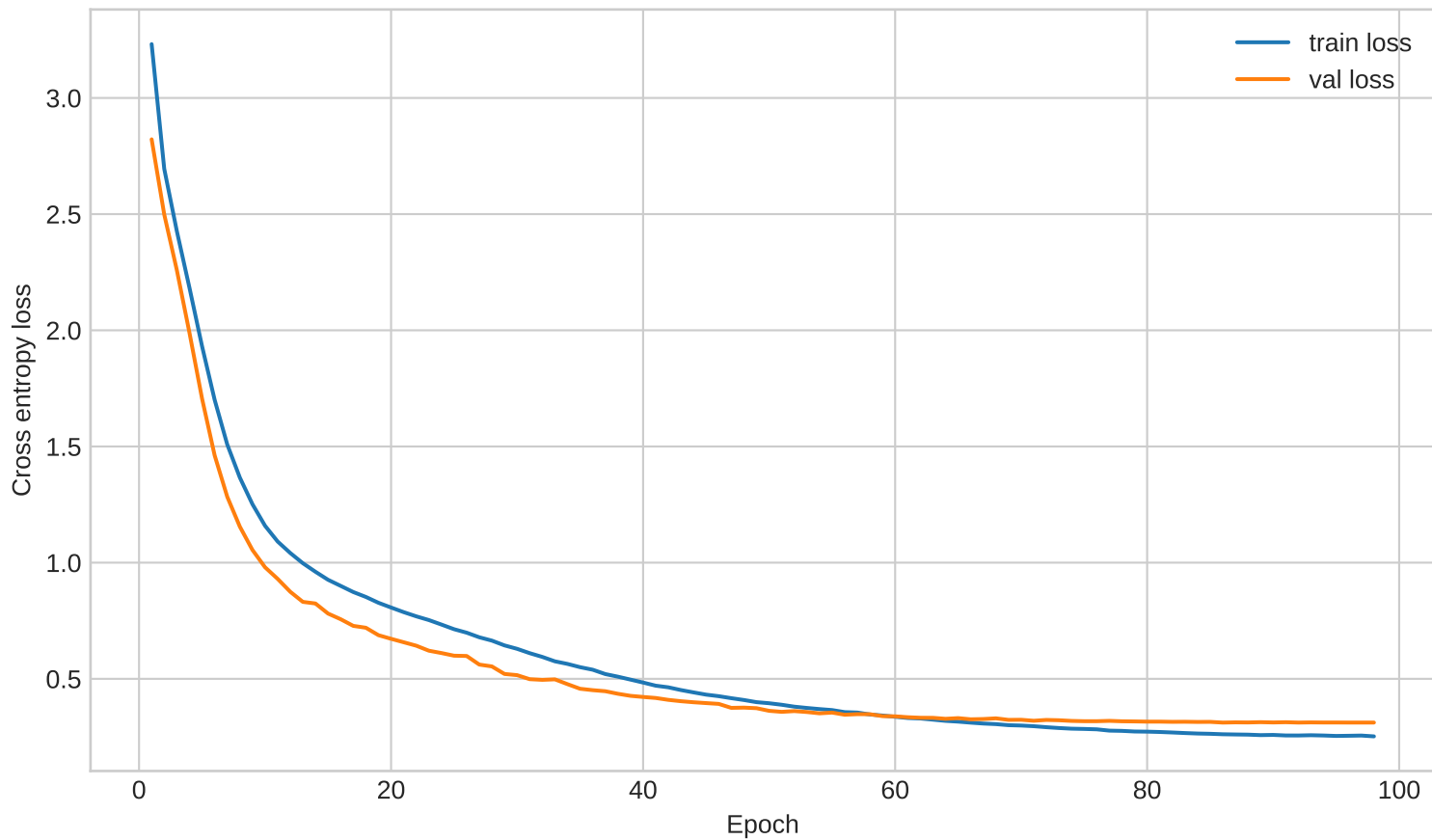
Arabic-with-Levanti-harakat to Arabizi loss
