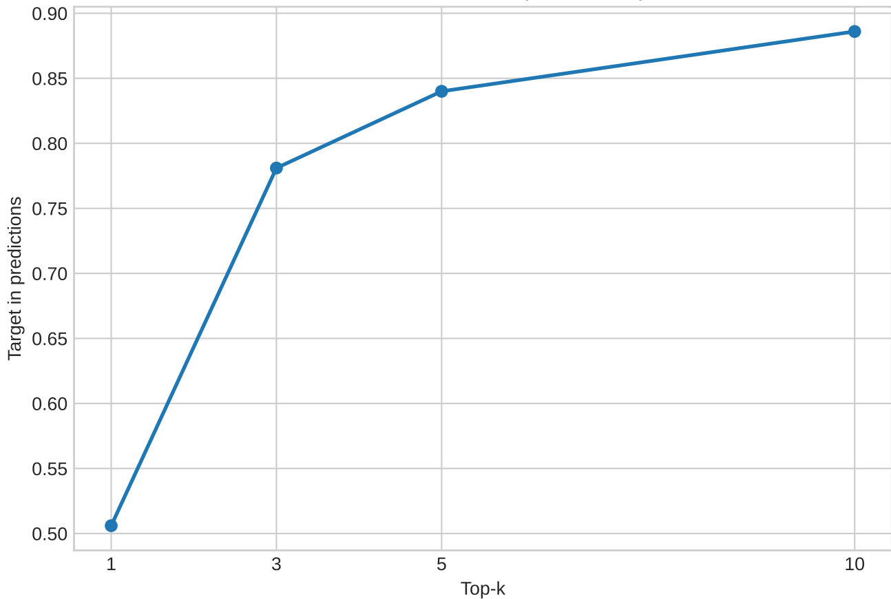
Softmax 90 Arabizi top-k accuracy
