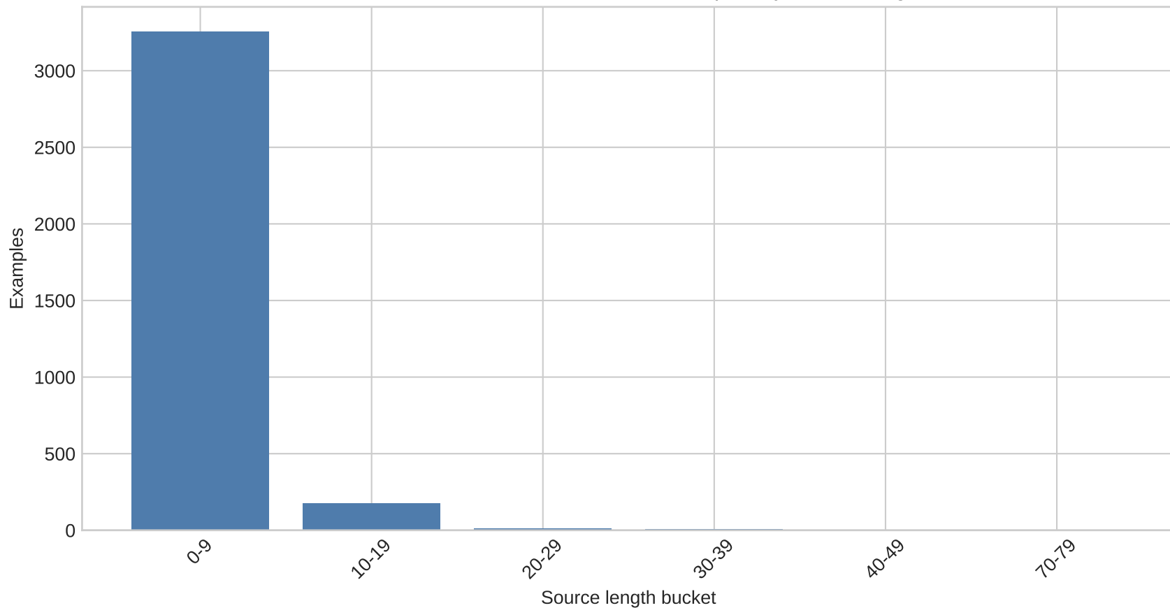
Arabic-without-harakat to Arabizi examples by source length
