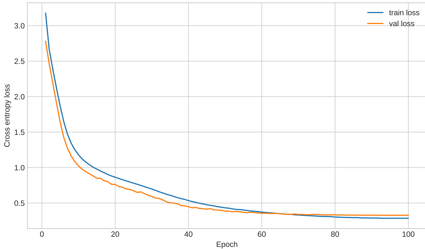
Arabic-without-harakat to Arabizi loss
