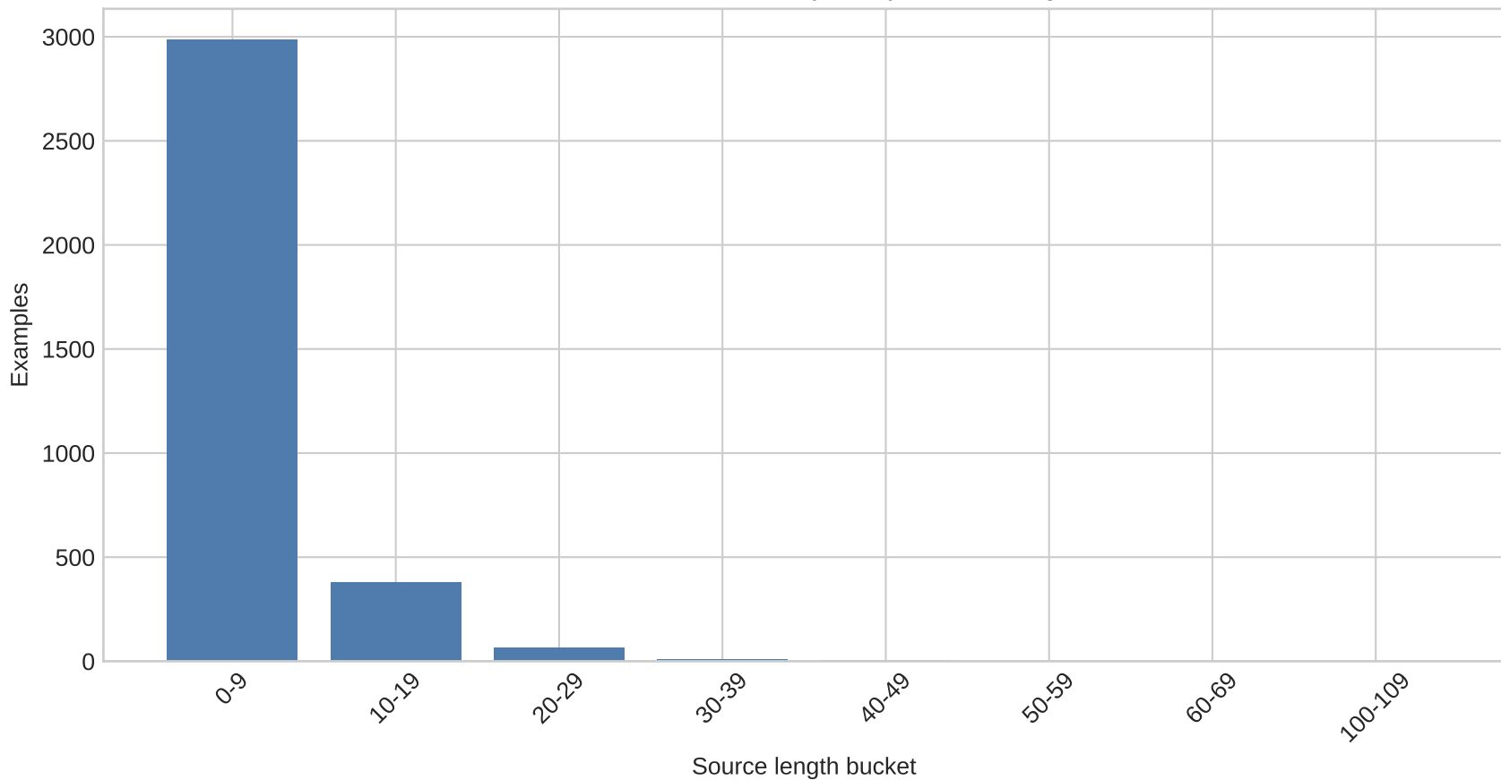
Arabizi to Arabic examples by source length
