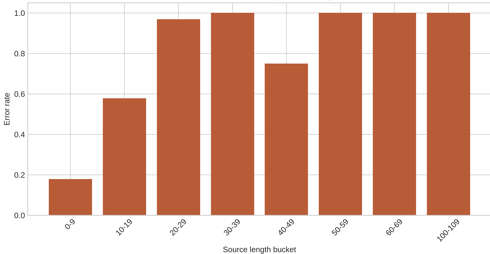
Arabizi to Arabic error by source length
