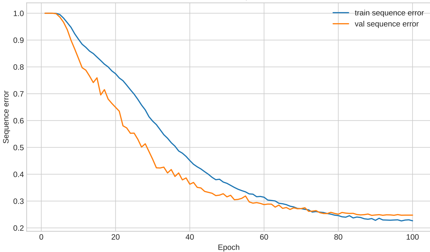
Arabizi to Arabic sequence error
