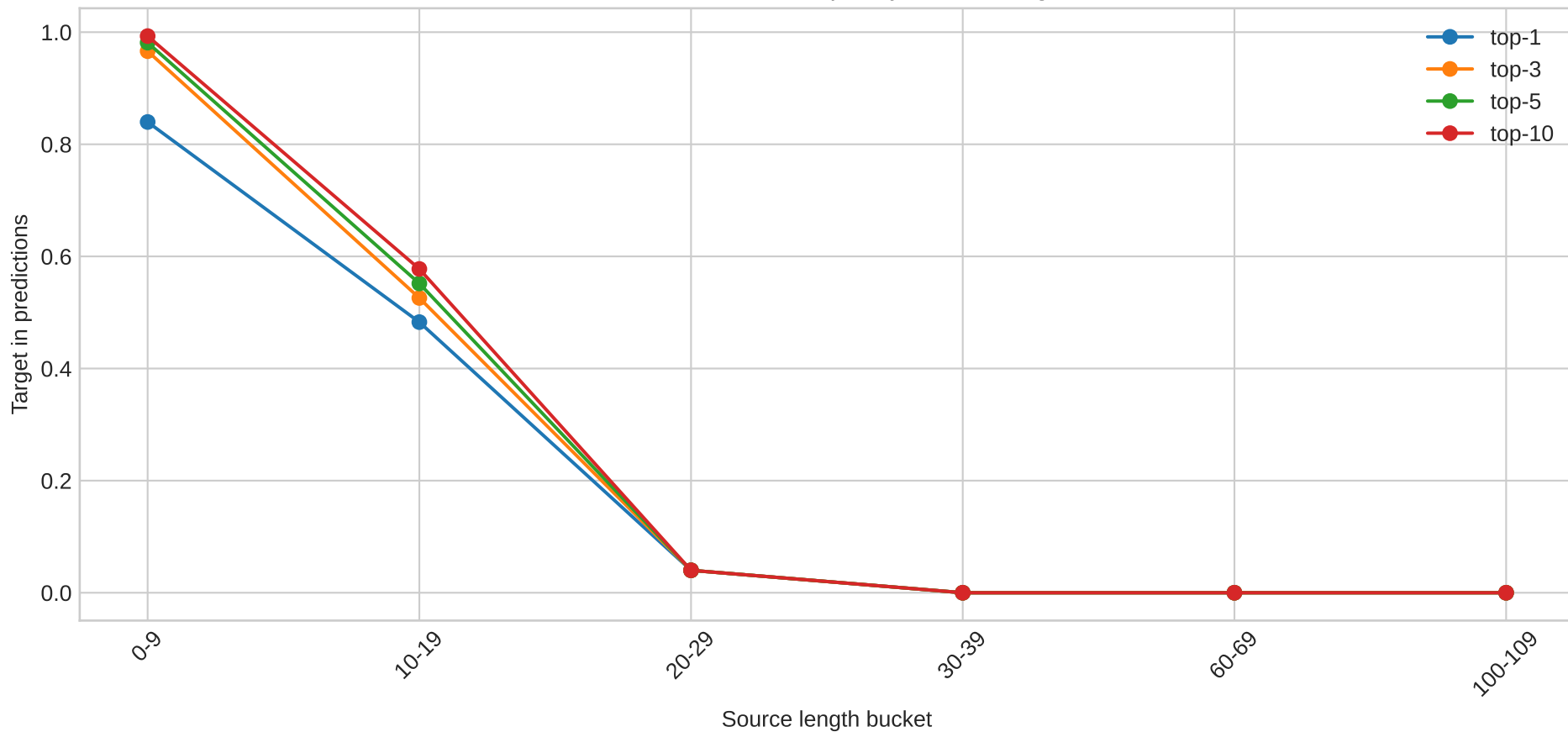
Softmax 90 Arabic top-k by source length
