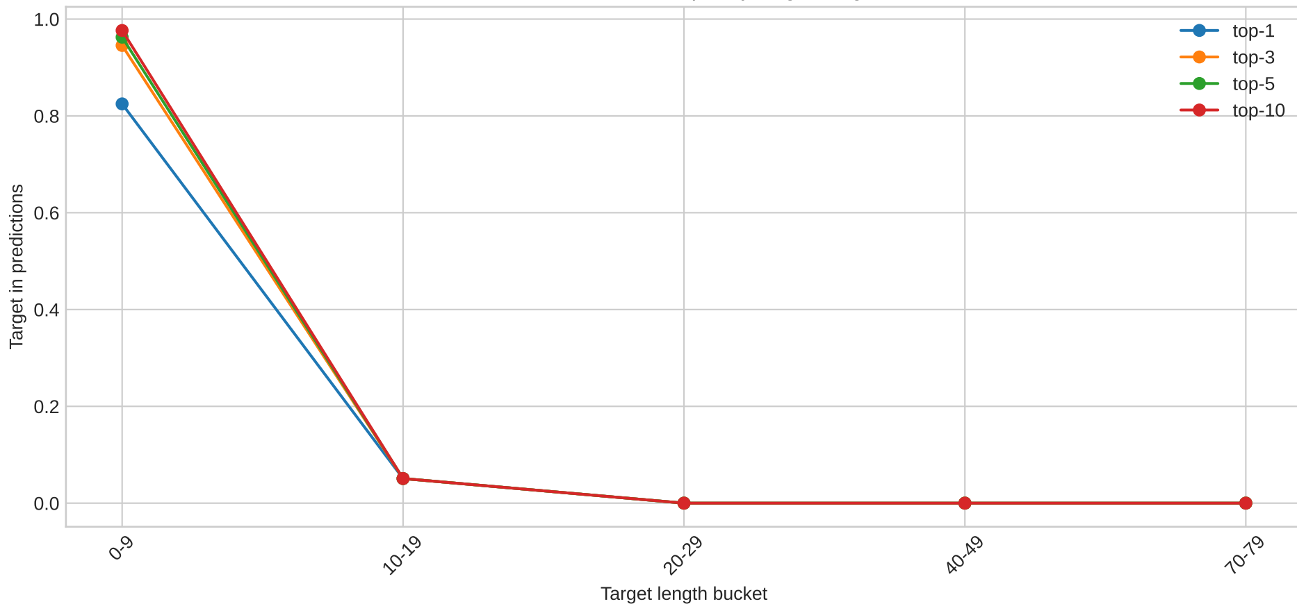
Softmax 90 Arabic top-k by target length
