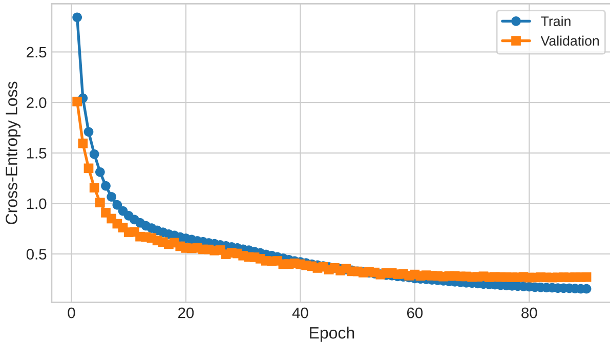
Cross-Entropy Error During Harakat Adder Training
