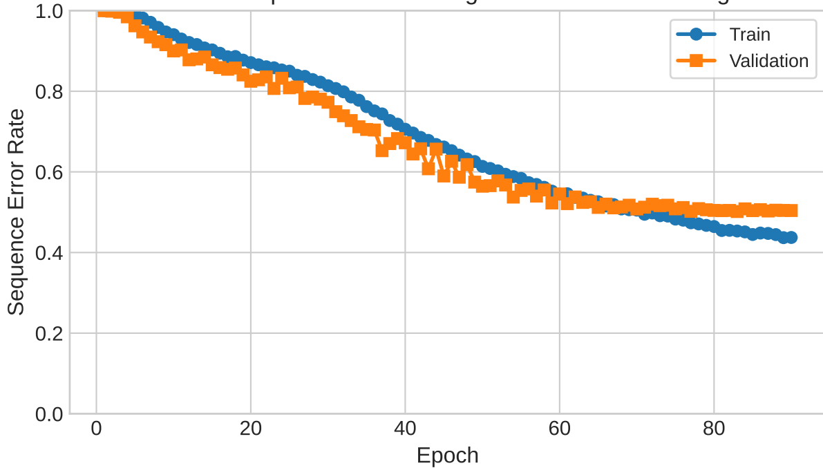
Exact-Sequence Error During Harakat Adder Training
