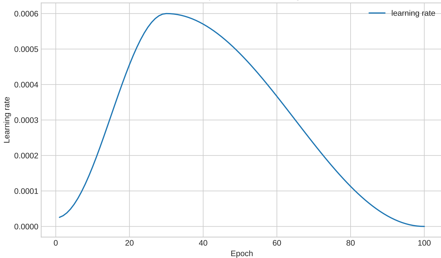
Harakat-top-1 to Arabizi learning rate
