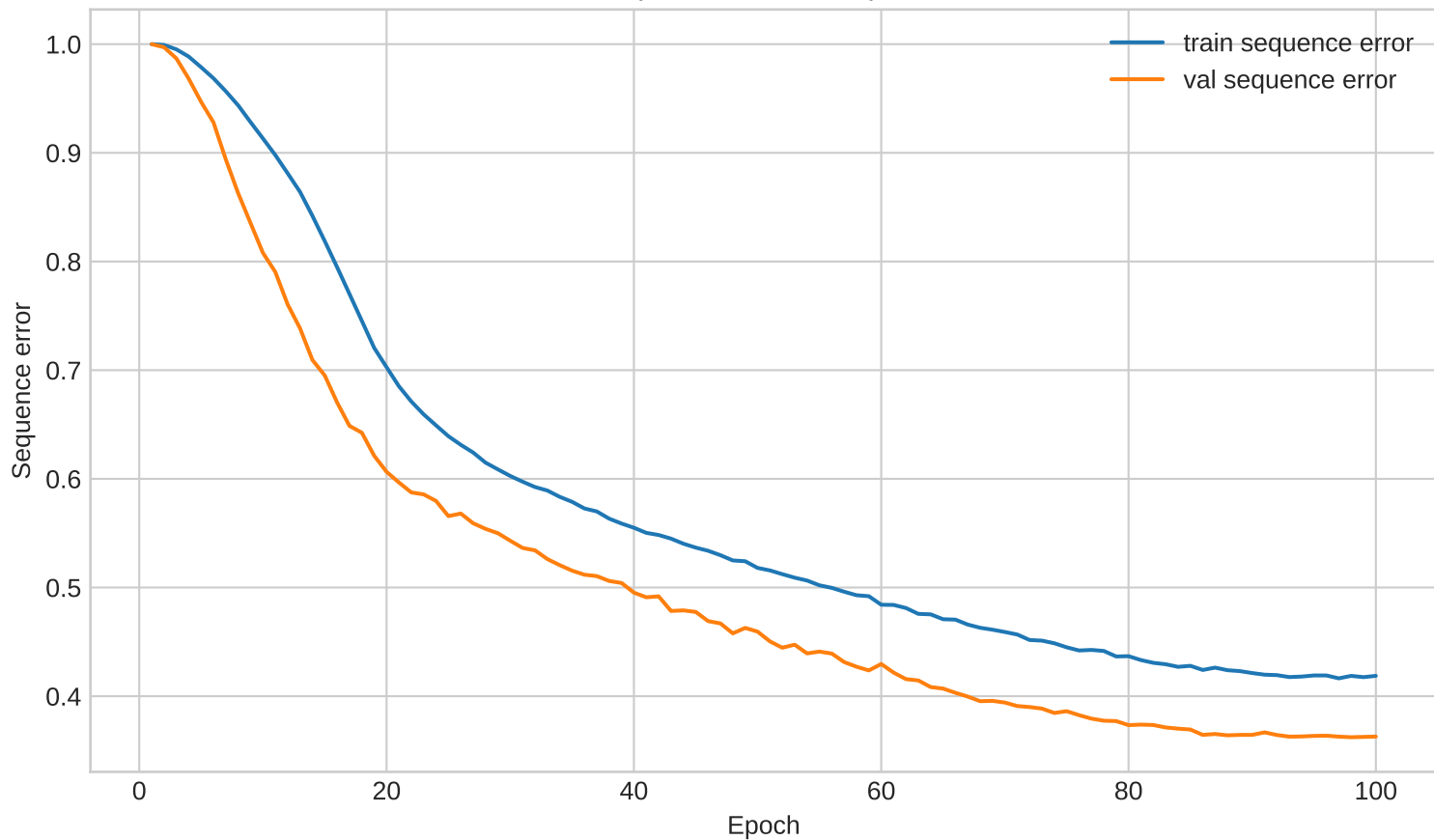
Harakat top 5 to Arabizi sequence error
