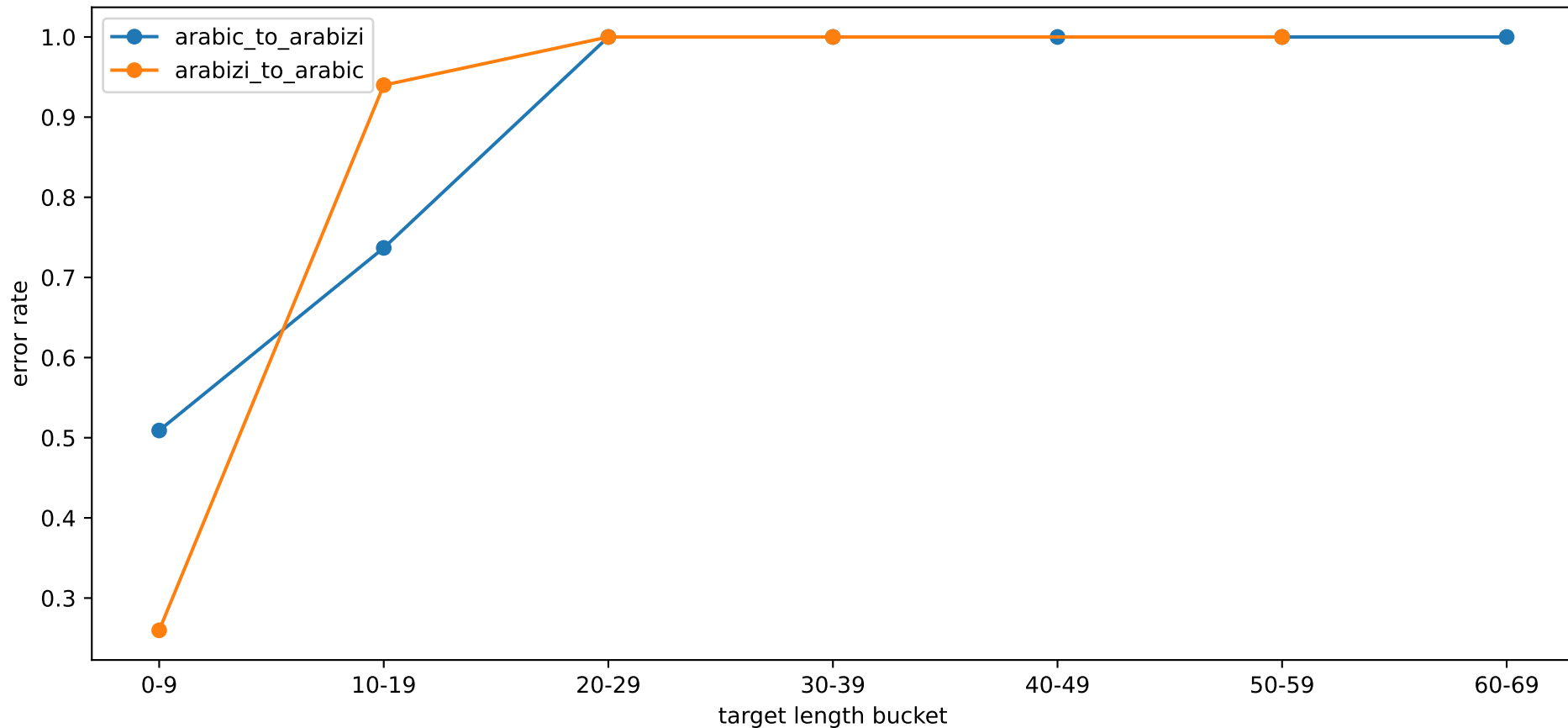
Shared bidirectional error by target length
