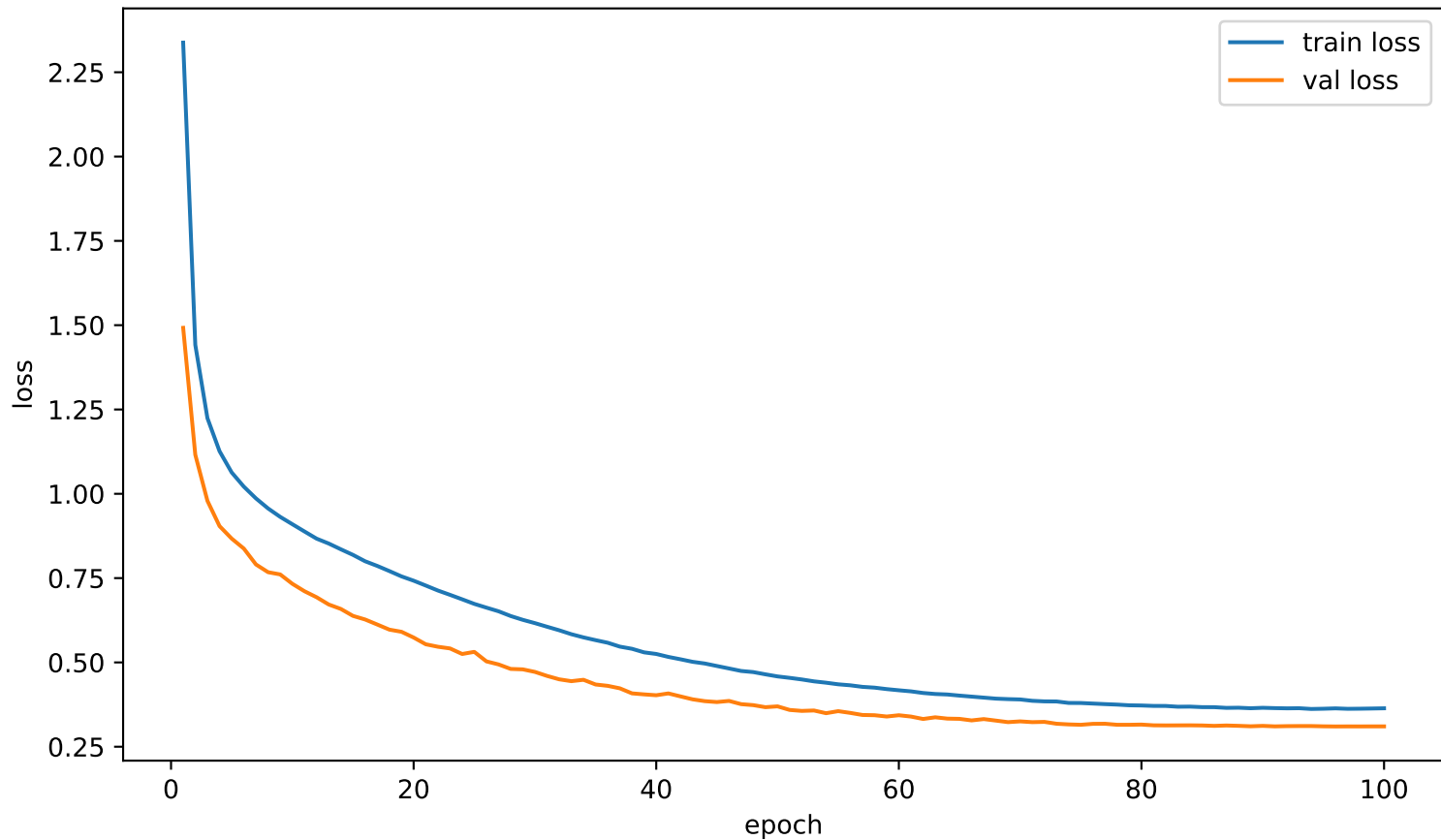
Shared bidirectional loss
