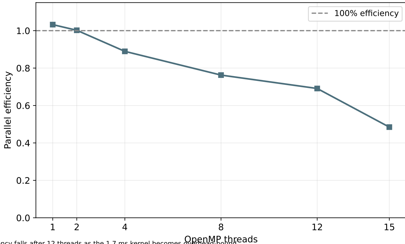
OpenMP efficiency (speedup / threads)
