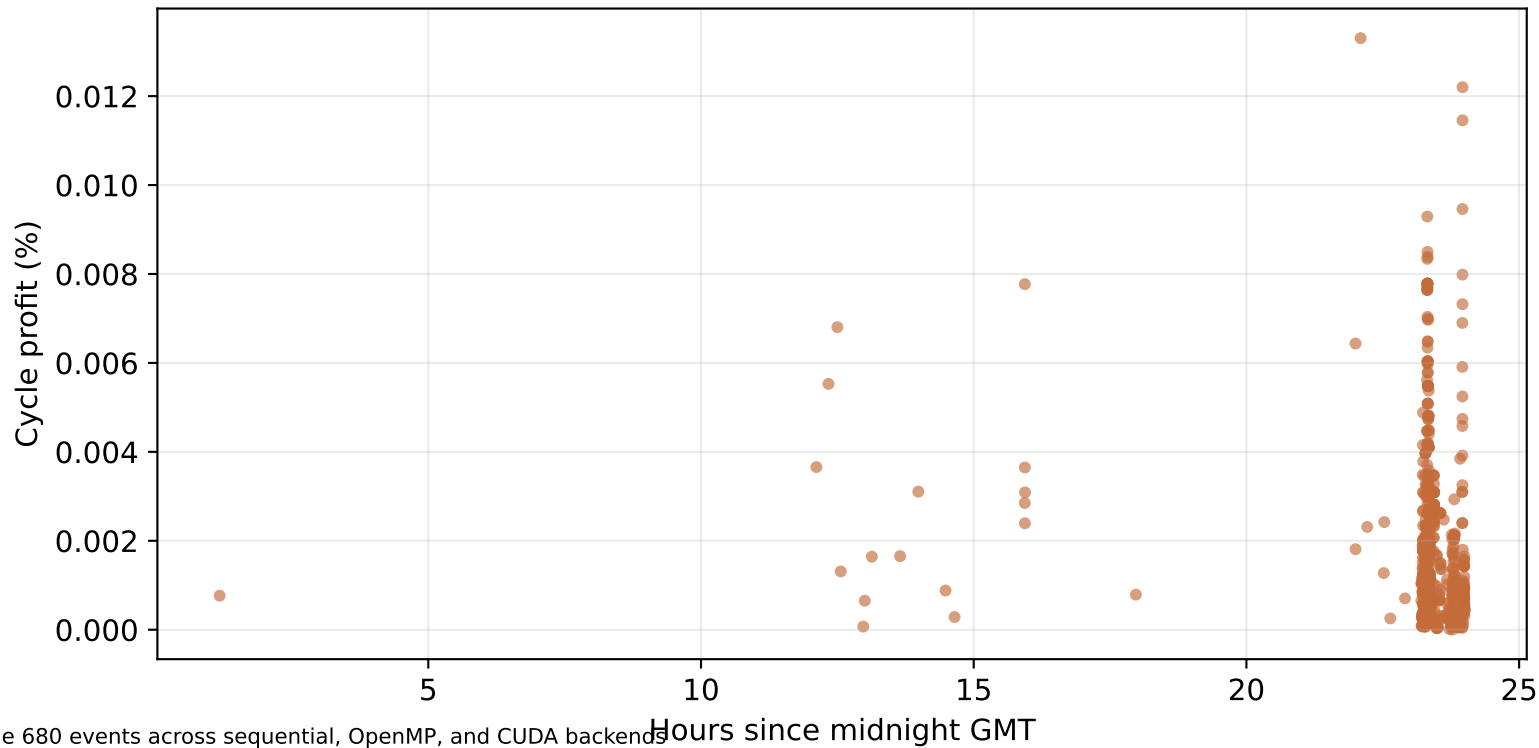
Intraday location of detected FX arbitrage cycles
