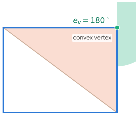
(a) convex: saturates at 180^\circ for every D_{\max}
