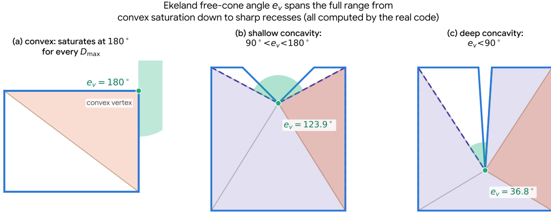
Figure 2: Ekeland free-cone angle geometry across its full range, three cases (all computed by the actual kernel-expansion code, not hand-derived). (a) A convex vertex: the free cone (green) saturates at e_v = 180^\circ at every expansion depth D_{\max} , since no merge ever introduces a reflex angle there—this is why a plain interior angle alone cannot discriminate convex corners, motivating the free-space term. (b) A shallow, obtuse recess (grey CDT mesh; seed triangle orange; P_{\text{sub}} violet after 2 merges): the free cone is compressed but still wide, e_v = 123.9^\circ \in (90^\circ, 180^\circ) . (c) A sharp, acute recess (same construction, 3 merges): the free cone narrows well past the halfway point, e_v = 36.8^\circ < 90^\circ . Together the three cases span the descriptor’s full range from convex saturation to a sharp recess; how quickly a given recess surfaces also depends on where CDT happens to place the seed triangle relative to it, which is why D_{\max} is swept empirically rather than fixed by assumption (Section 6.7). Three such scalars, one per triangle vertex, form the free-space sub-vector (e_1, e_2, e_3) of the 5-D descriptor f = (\alpha_1, \alpha_2, e_1, e_2, e_3) .
