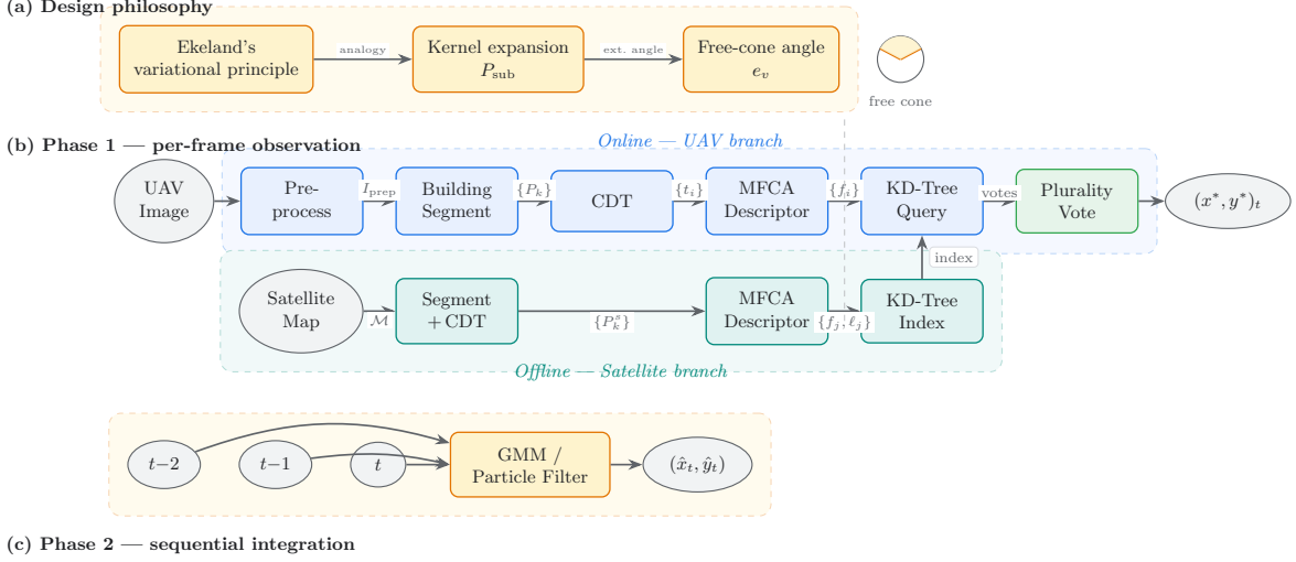
Figure 1: Method overview. (a) Design philosophy: Ekeland’s variational principle motivates a kernel expansion P_{\text{sub}} —a maximal merge of adjacent CDT triangles—whose exterior angle at each vertex, the free-cone angle e_v , is bounded away from both 0^\circ and the saturated 180^\circ convex value, making it discriminative (Figure 2 illustrates this on concrete cases). (b) Phase 1 turns a single UAV image into a per-frame observation: the online branch (blue) extracts the 5-D descriptor and queries the offline satellite index (teal) built once per map site; plurality voting yields a per-frame position estimate (x^*, y^*)_t . (c) Phase 2 integrates these per-frame estimates across a trajectory with a Gaussian-mixture/particle filter (Section 5.8), producing a refined position (\hat{x}_t, \hat{y}_t) —though Section 6.8 shows this integration step cannot recover accuracy the per-frame observation never had.
