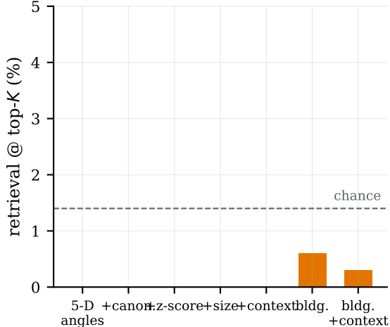
(b) yet retrieval stays \approx 0\%
