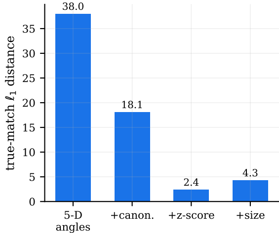
(a) enrichment shrinks the true-match distance ( 16 \times )
