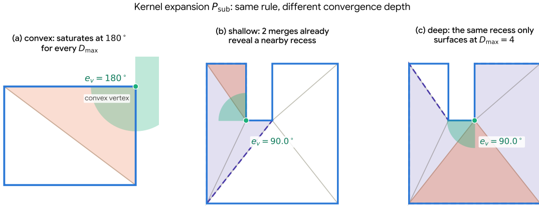
Figure 2: Ekeland free-cone angle geometry, three cases (all computed by the actual kernel-expansion code, not hand-derived). (a) A convex vertex: the free cone (green) saturates at e_v = 180^\circ at every expansion depth D_{\text{max}} , since no merge ever introduces a reflex angle there—this is why a plain interior angle alone cannot discriminate convex corners, motivating the free-space term. (b) A vertex whose true concavity (a rectangular recess, grey CDT mesh) is revealed quickly : the seed triangle (orange) already sits against the recess, so 2 merges (violet P_{\text{sub}} , dashed boundary) suffice to reach the converged value e_v = 90^\circ . (c) The same recess, approached from a different seed triangle (orange, far side of the shape): P_{\text{sub}} must absorb every interior triangle before the angle at the shared vertex drops from the naive 180^\circ to the same true e_v = 90^\circ , only at the full budget D_{\text{max}} = 4 . (b) vs. (c) is why D_{\text{max}} is swept empirically rather than fixed by assumption (Section 6.7): the same geometric feature can need anywhere from one merge to the full budget to surface, depending on where CDT happens to place the seed triangle. Three such scalars, one per triangle vertex, form the free-space sub-vector (e_1, e_2, e_3) of the 5-D descriptor f = (\alpha_1, \alpha_2, e_1, e_2, e_3) .
