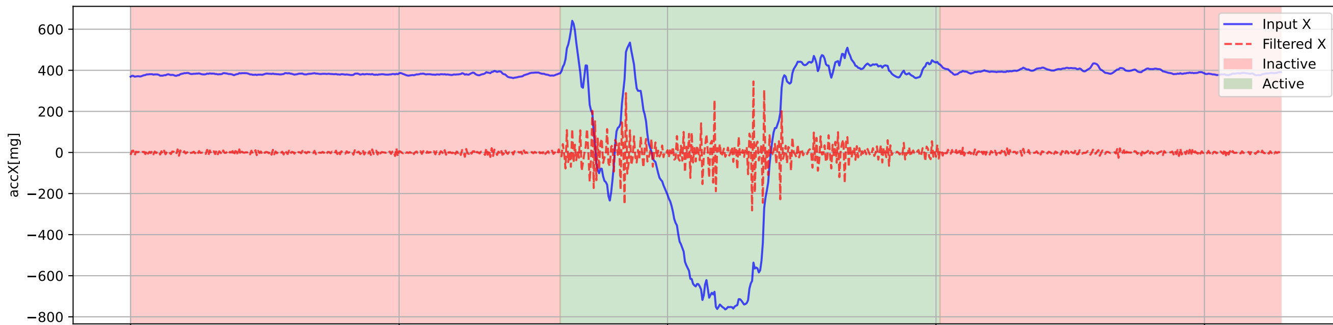
Accelerometer X-axis
