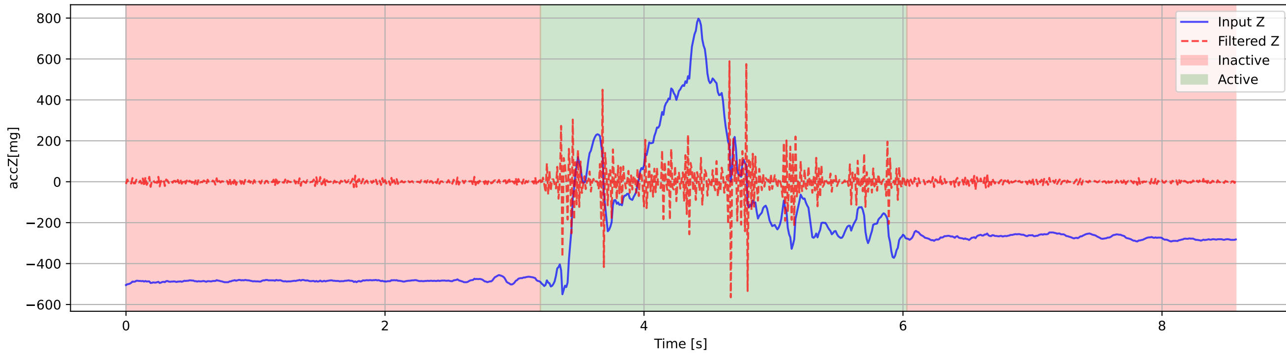
Accelerometer Z-axis
