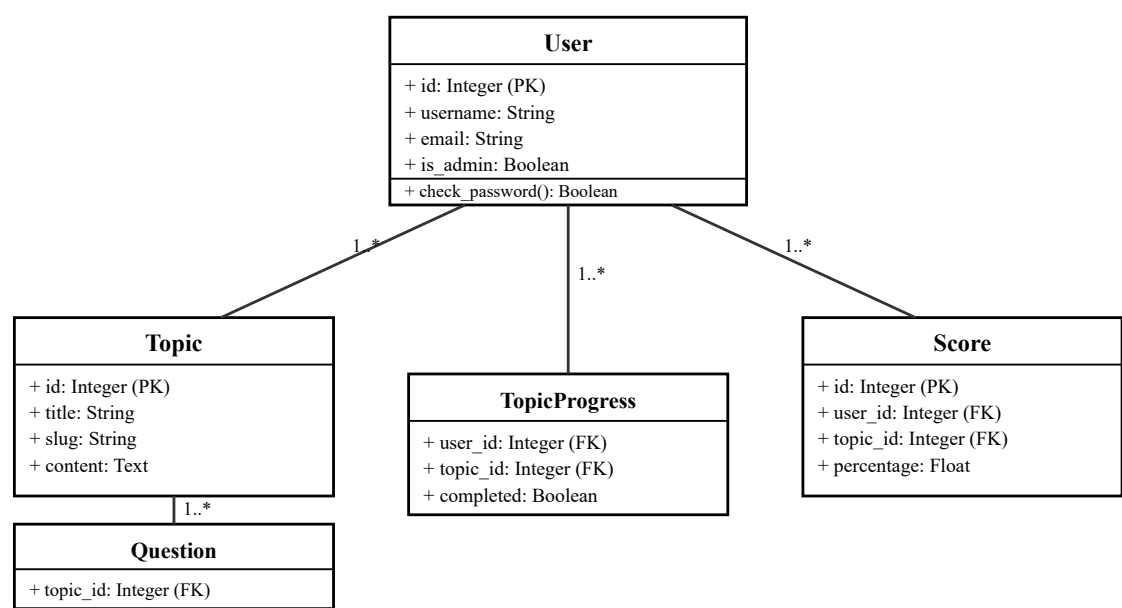
Figure 4.7: UML Class Diagram “Data Entities & Method Signatures
