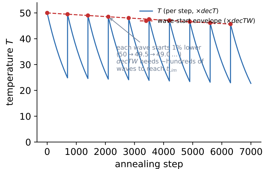
Phase 1 temperature (waves)
