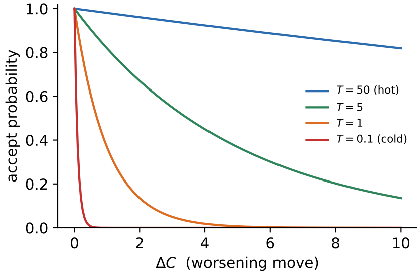
Metropolis acceptance e^{-\Delta C/T}
