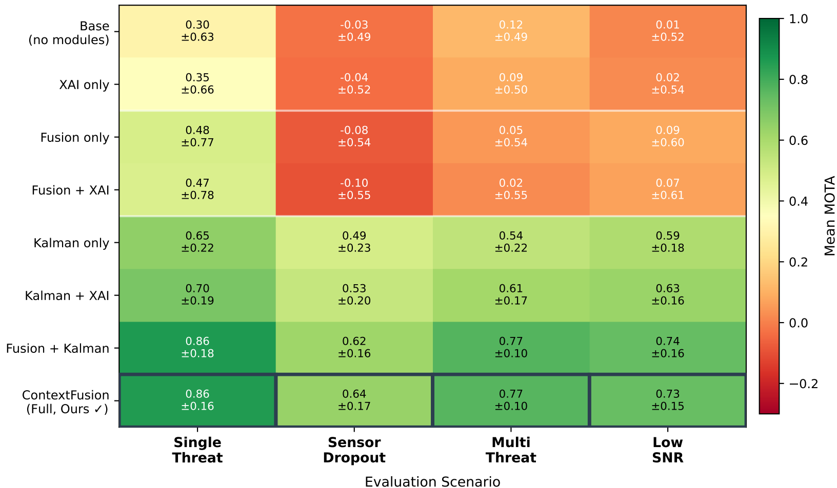
Ablation Study — Mean MOTA per Configuration and Scenario
