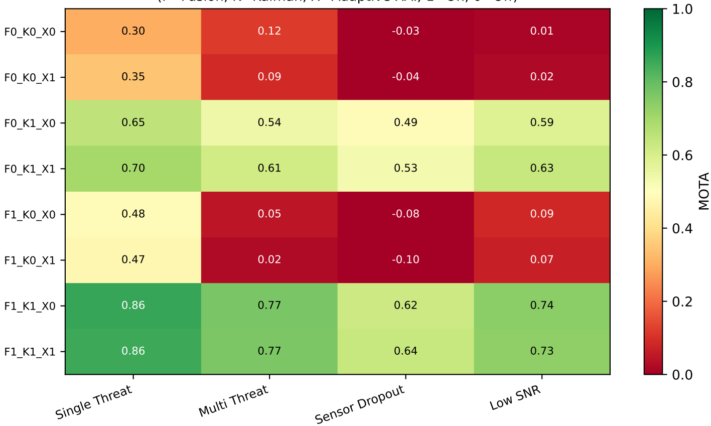
Ablation Study — MOTA Heatmap (F=Fusion, K=Kalman, X=Adaptive XAI; 1=On, 0=Off)
