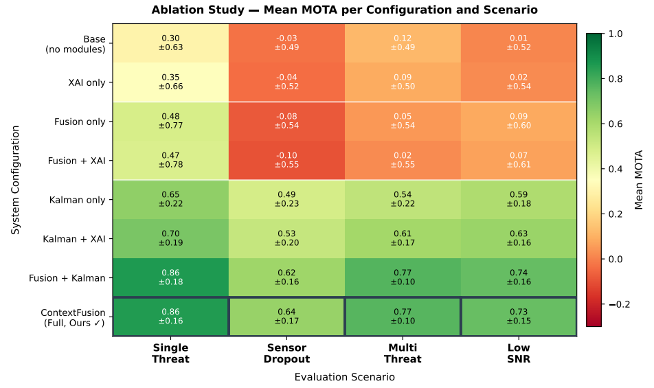
Figure 3. Ablation heatmap: mean MOTA per configuration and scenario. Green = high MOTA; red = low. Rows ordered by performance.
